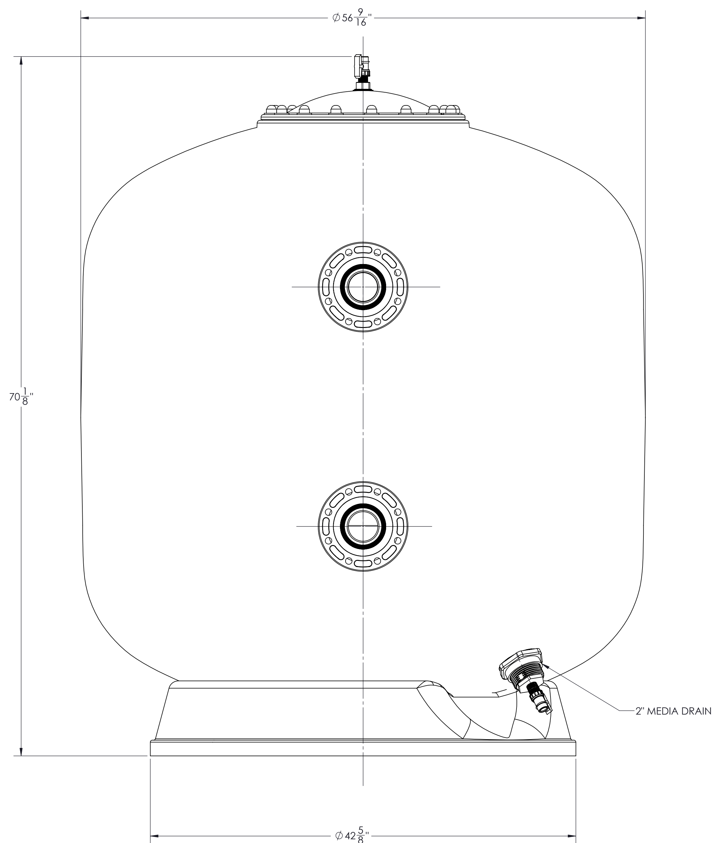
VERTICAL SAND FILTER WITH 4" CONNECTION
